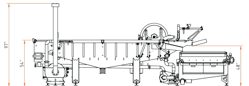
Dimensional sketch based on the PULSTAR-100 version
